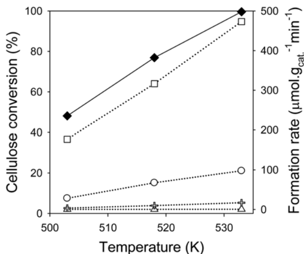
Fig. 5. Variations of the cellulose conversion and the formation rate of various gaseous products at different reaction temperature over Pt/H-ZSM-5(150). Left-hand axis: conversion of cellulose (◆); right-hand axis: formation rates of H_2 (○), CO_2 (□), CO (△) and CH_4 (+). Reaction conditions: the weight of cellulose=0.99 g, the weight of water=45 g, the weight of catalyst=0.10 g; reaction time=1 h, 1 vol% N_2/He pressure=1 MPa.
